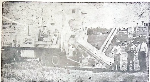
A new concept in Livestock Feeds processing and manufacturing that can start making money for its investors immediately. The unit, mounted on a lorry goes to any location, grinds, mixes and weighs any feedstuffs, makes any size pellet to any desired formula at savings up to four pounds per ton or more. The Nigeria's representatives of the dealers are Messrs Shonubi Stores Ltd. P. O. Box 1039, Yaba.
