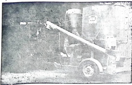
A mixer which incorporates a hammer mill with a plain feed table, ladder, 10ft discharge conveyor, universal power take-off drive from the tractor, safety shear pin and discharge system clutch. The unit costs about £800.
